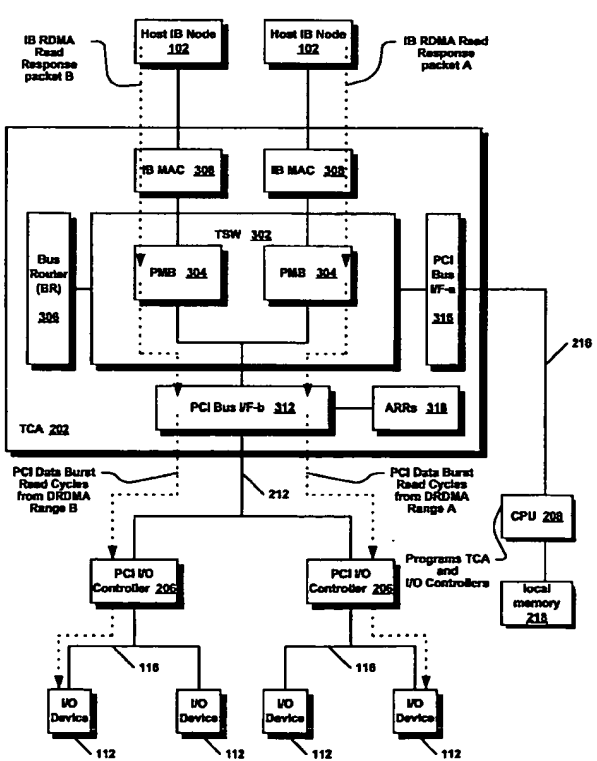
Direct RDMA Read Data Flow
